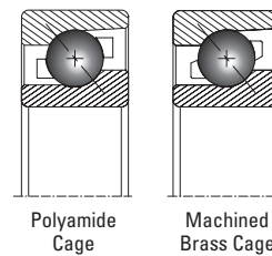
Fig. 1. Cage variants: single-row.
